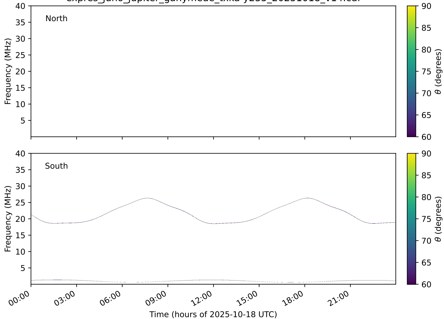
expres_juno_jupiter_ganymede_txka-y235_20251018_v14.cdf
