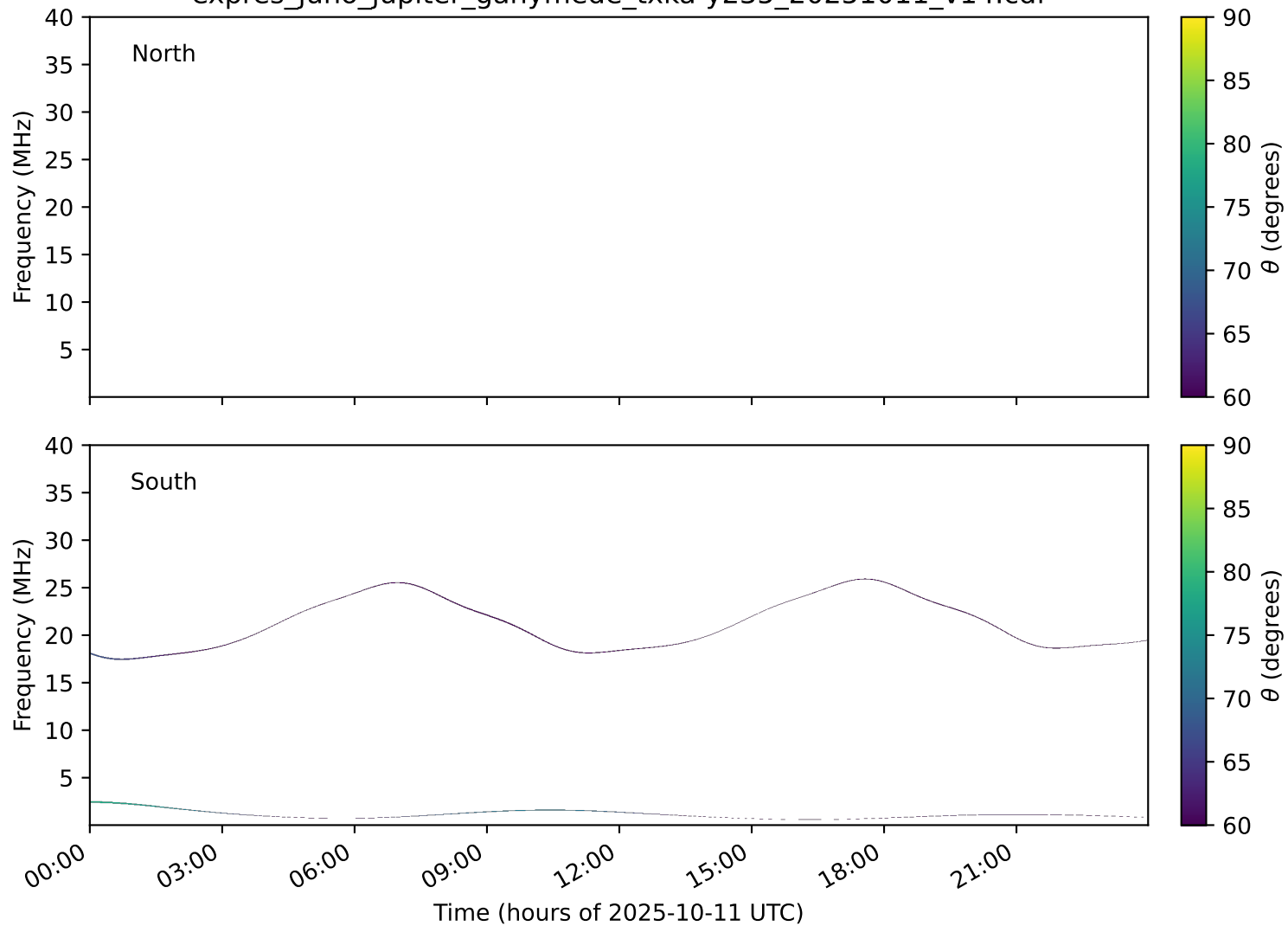
expres_juno_jupiter_ganymede_txka-y235_20251011_v14.cdf
