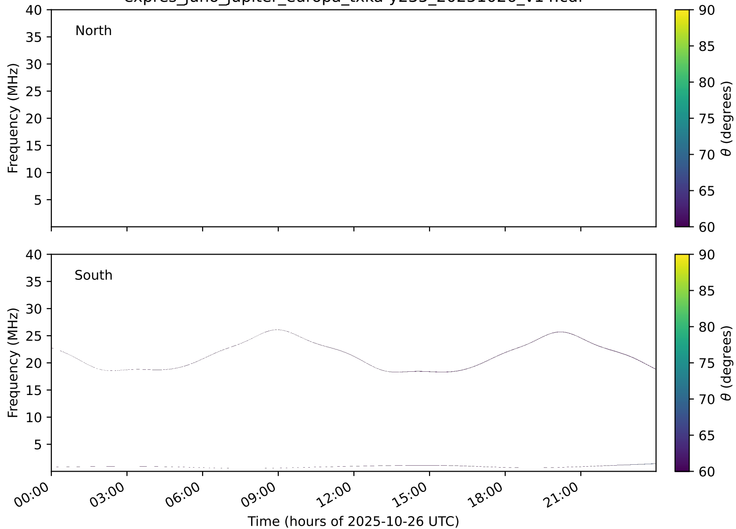
expres_juno_jupiter_europa_txka-y235_20251026_v14.cdf
