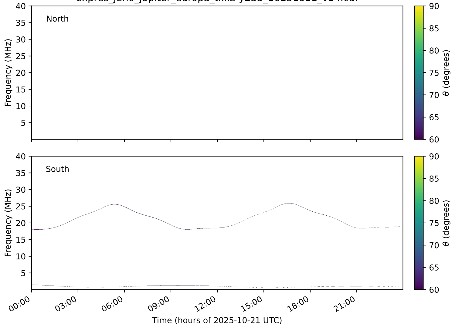
expres_juno_jupiter_europa_txka-y235_20251021_v14.cdf
