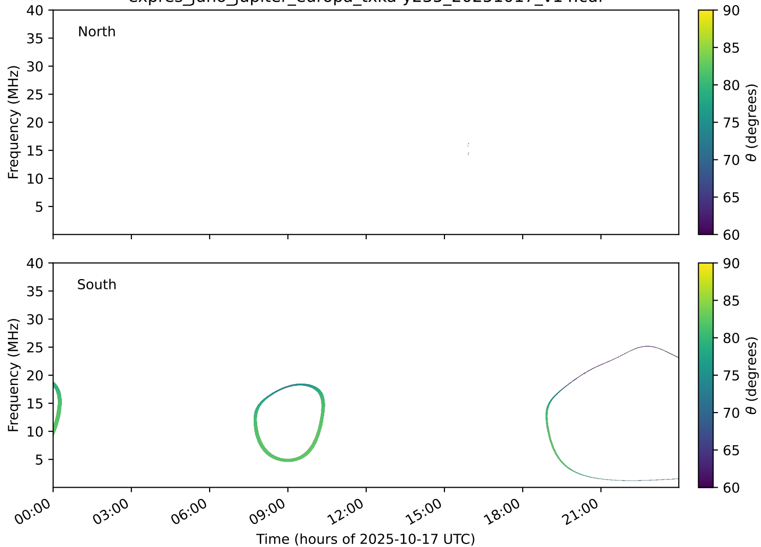
expres_juno_jupiter_europa_txka-y235_20251017_v14.cdf
