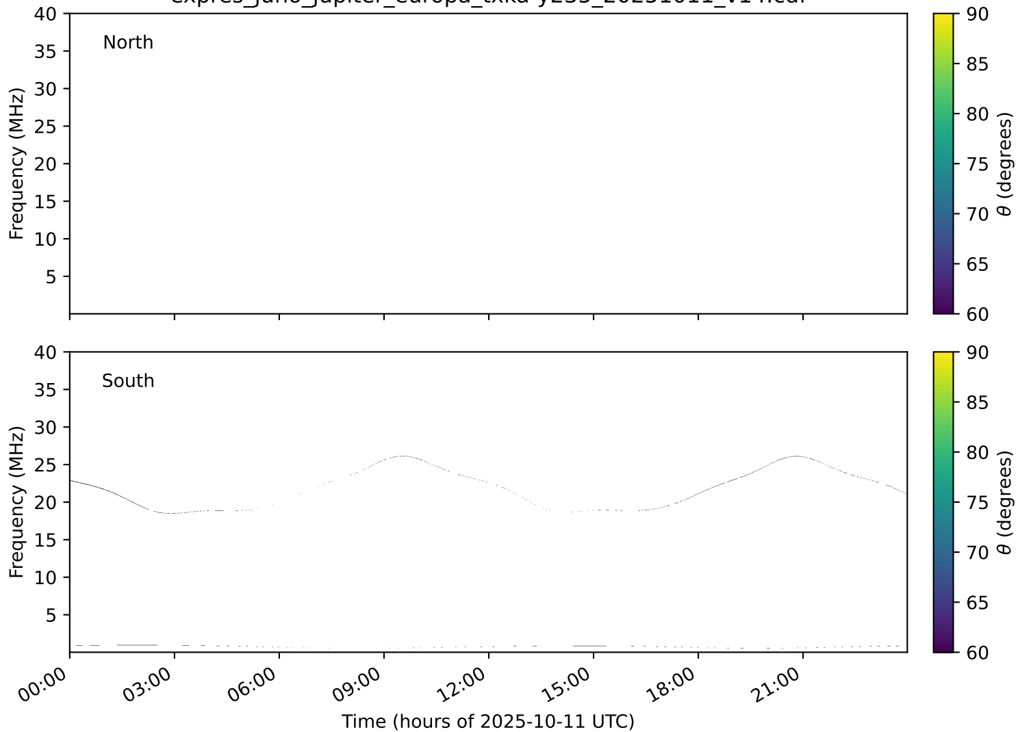
expres_juno_jupiter_europa_txka-y235_20251011_v14.cdf
