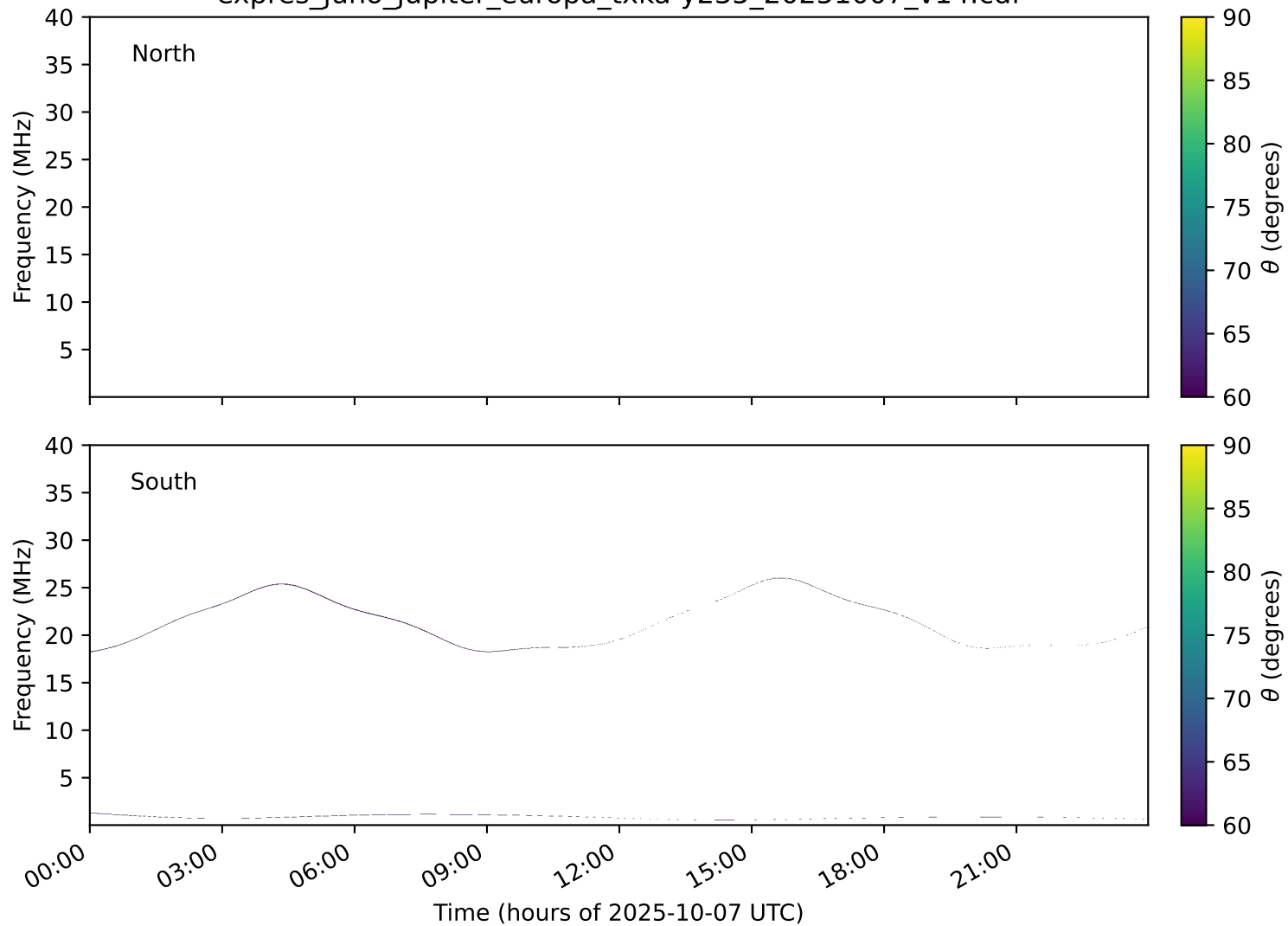
expres_juno_jupiter_europa_txka-y235_20251007_v14.cdf
