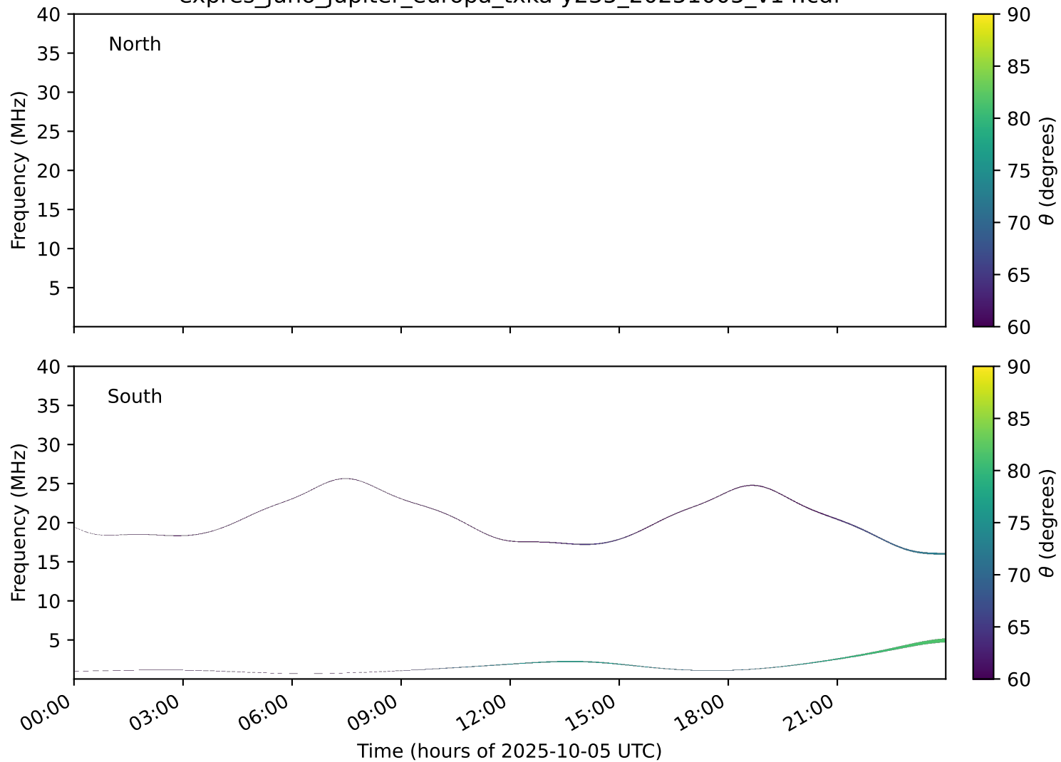
expres_juno_jupiter_europa_txka-y235_20251005_v14.cdf
