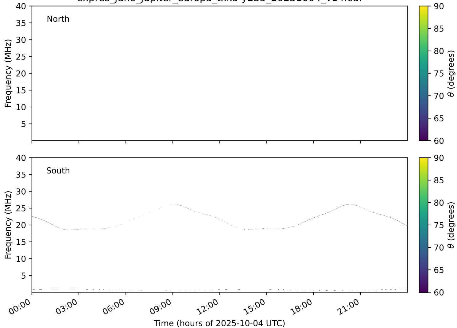
expres_juno_jupiter_europa_txka-y235_20251004_v14.cdf
