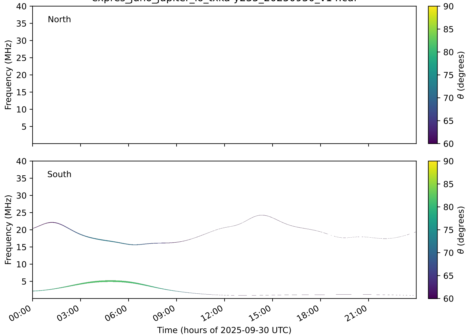
expres_juno_jupiter_io_txka-y235_20250930_v14.cdf
