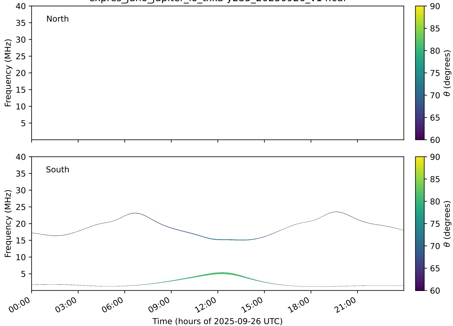
expres_juno_jupiter_io_txka-y235_20250926_v14.cdf
