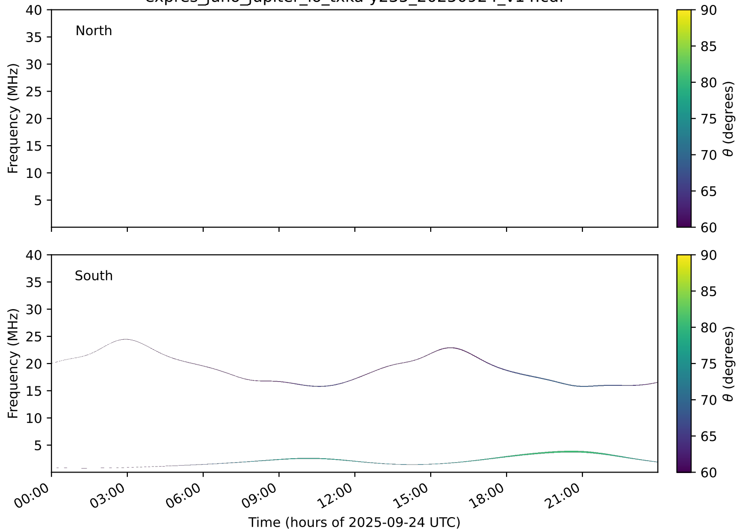
expres_juno_jupiter_io_txka-y235_20250924_v14.cdf
