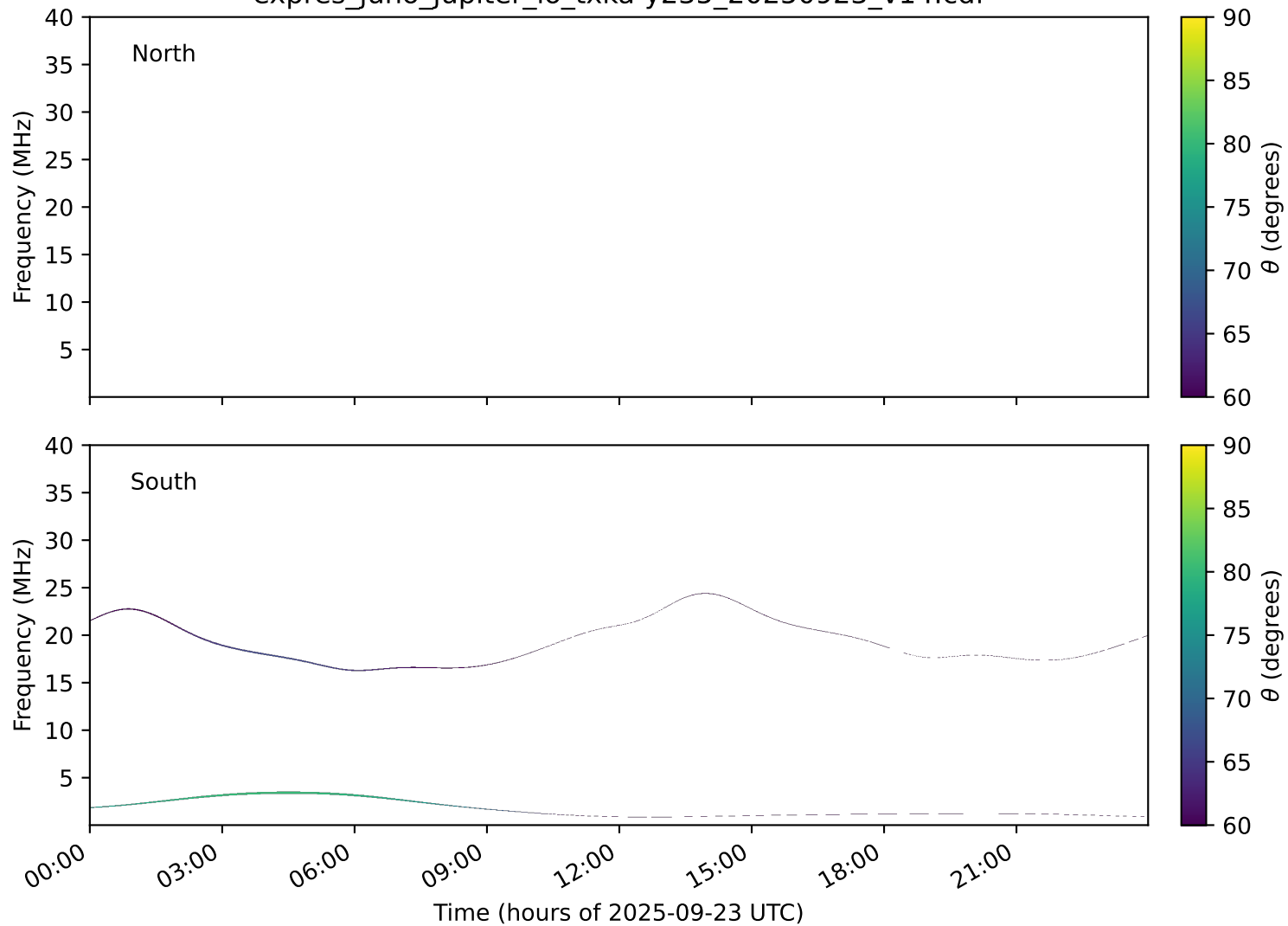
expres_juno_jupiter_io_txka-y235_20250923_v14.cdf
