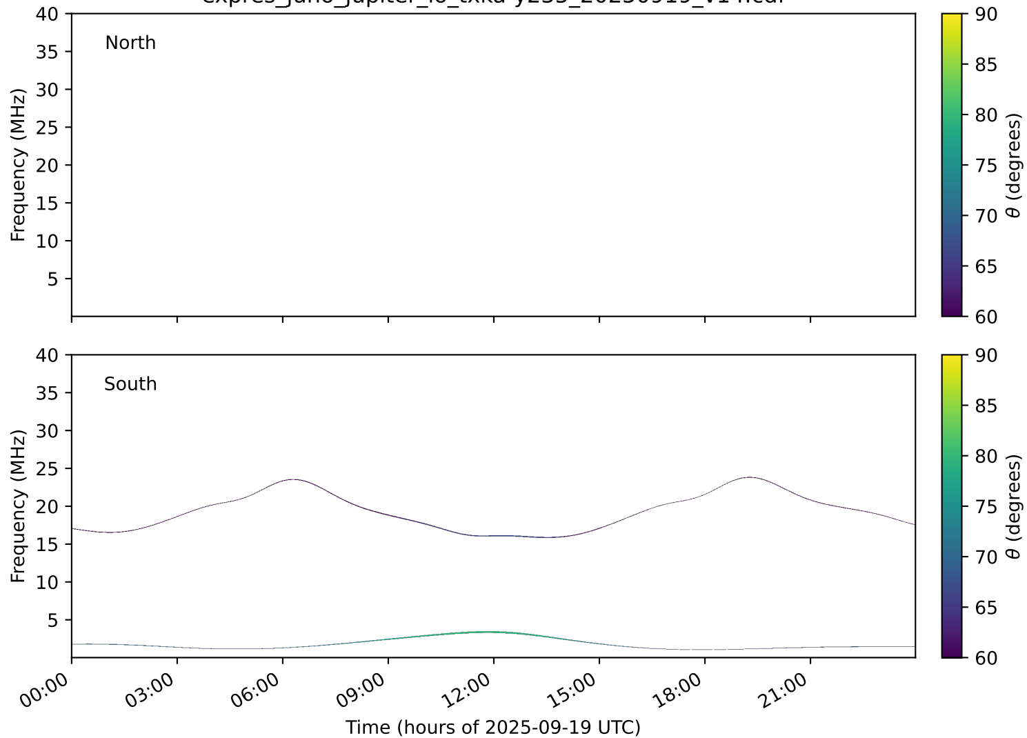
expres_juno_jupiter_io_txka-y235_20250919_v14.cdf
