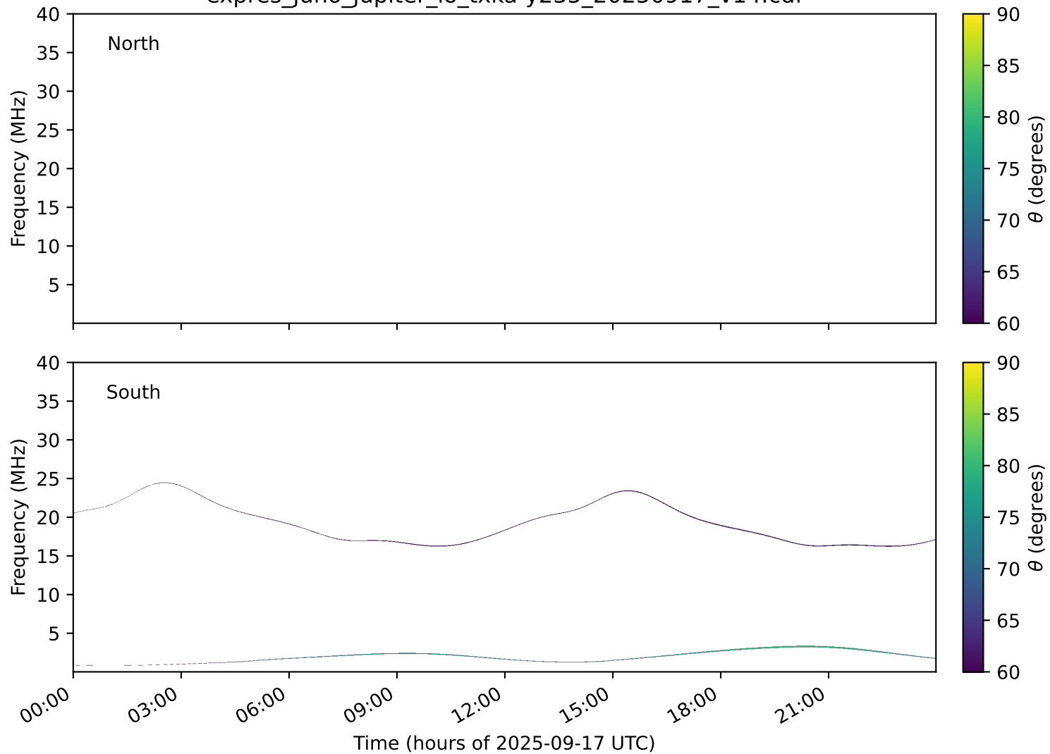
expres_juno_jupiter_io_txka-y235_20250917_v14.cdf
