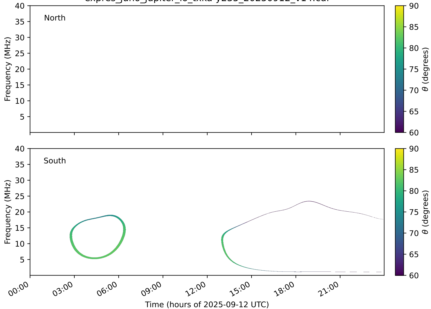
expres_juno_jupiter_io_txka-y235_20250912_v14.cdf
