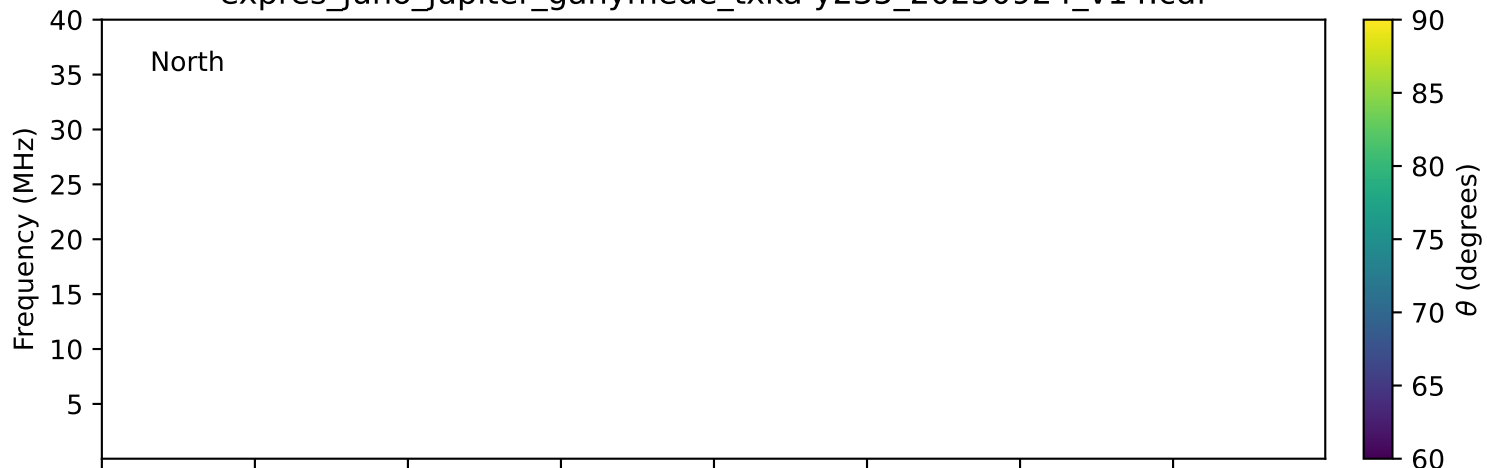
expres_juno_jupiter_ganymede_txka-y235_20250924_v14.cdf
