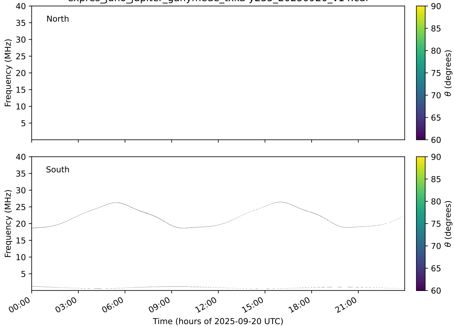
expres_juno_jupiter_ganymede_txka-y235_20250920_v14.cdf
