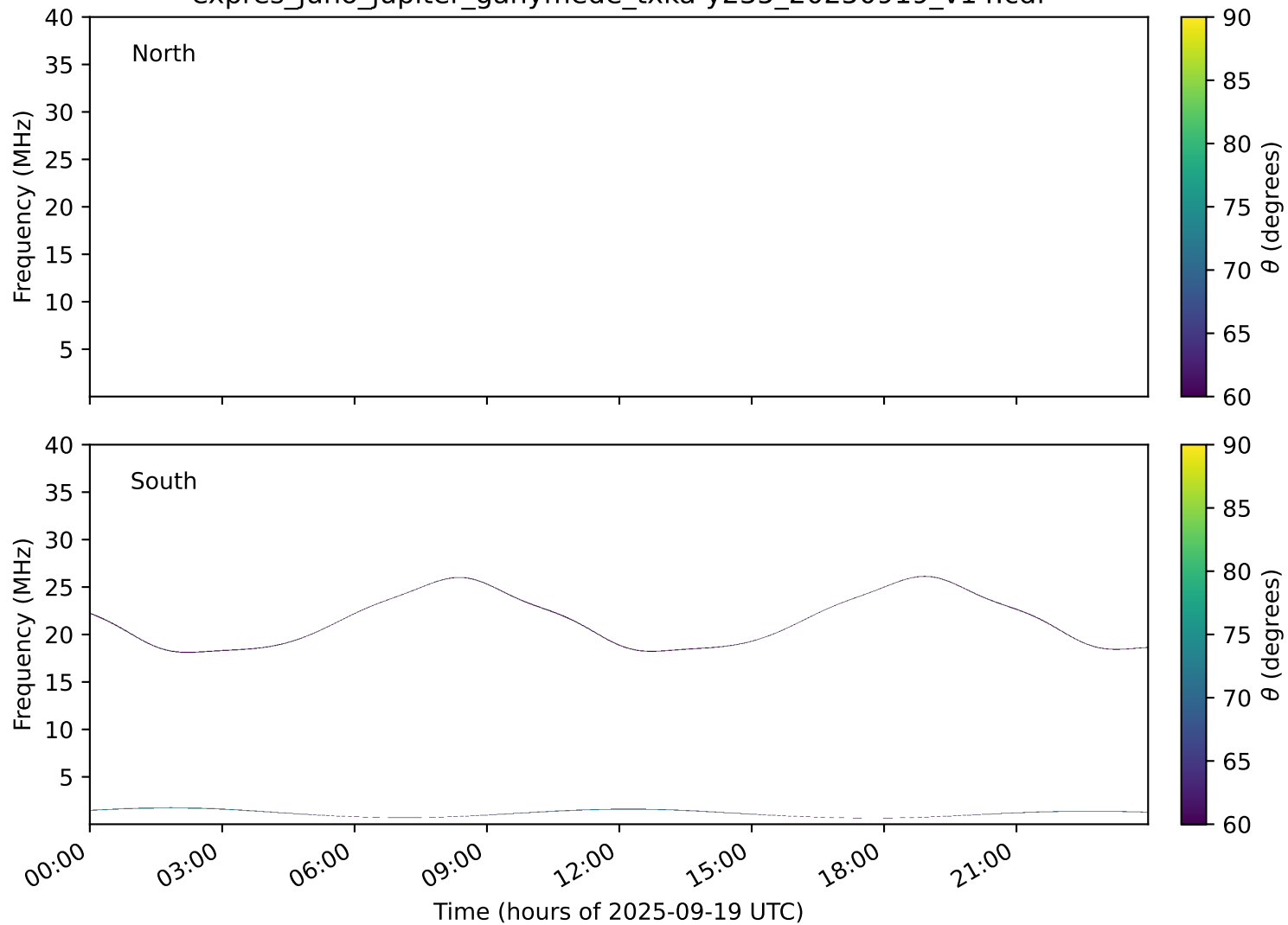
expres_juno_jupiter_ganymede_txka-y235_20250919_v14.cdf
