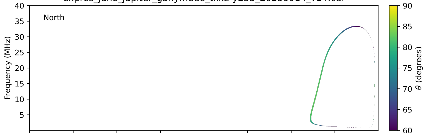
expres_juno_jupiter_ganymede_txka-y235_20250914_v14.cdf
