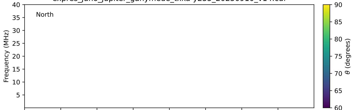
expres_juno_jupiter_ganymede_txka-y235_20250910_v14.cdf
