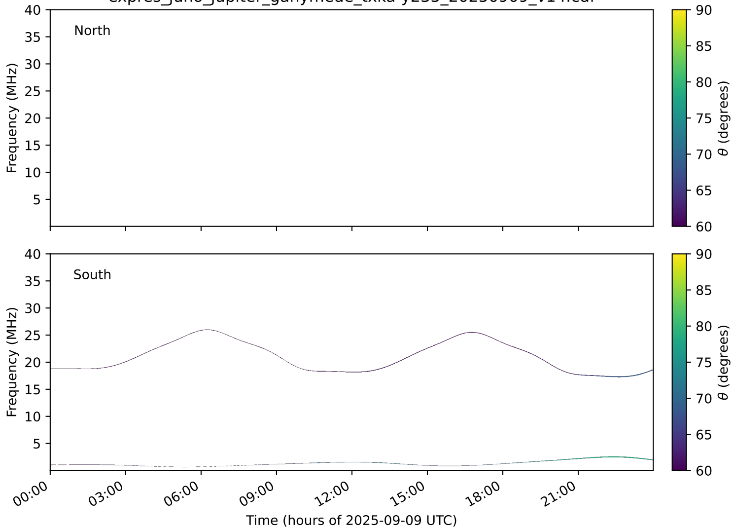
expres_juno_jupiter_ganymede_txka-y235_20250909_v14.cdf
