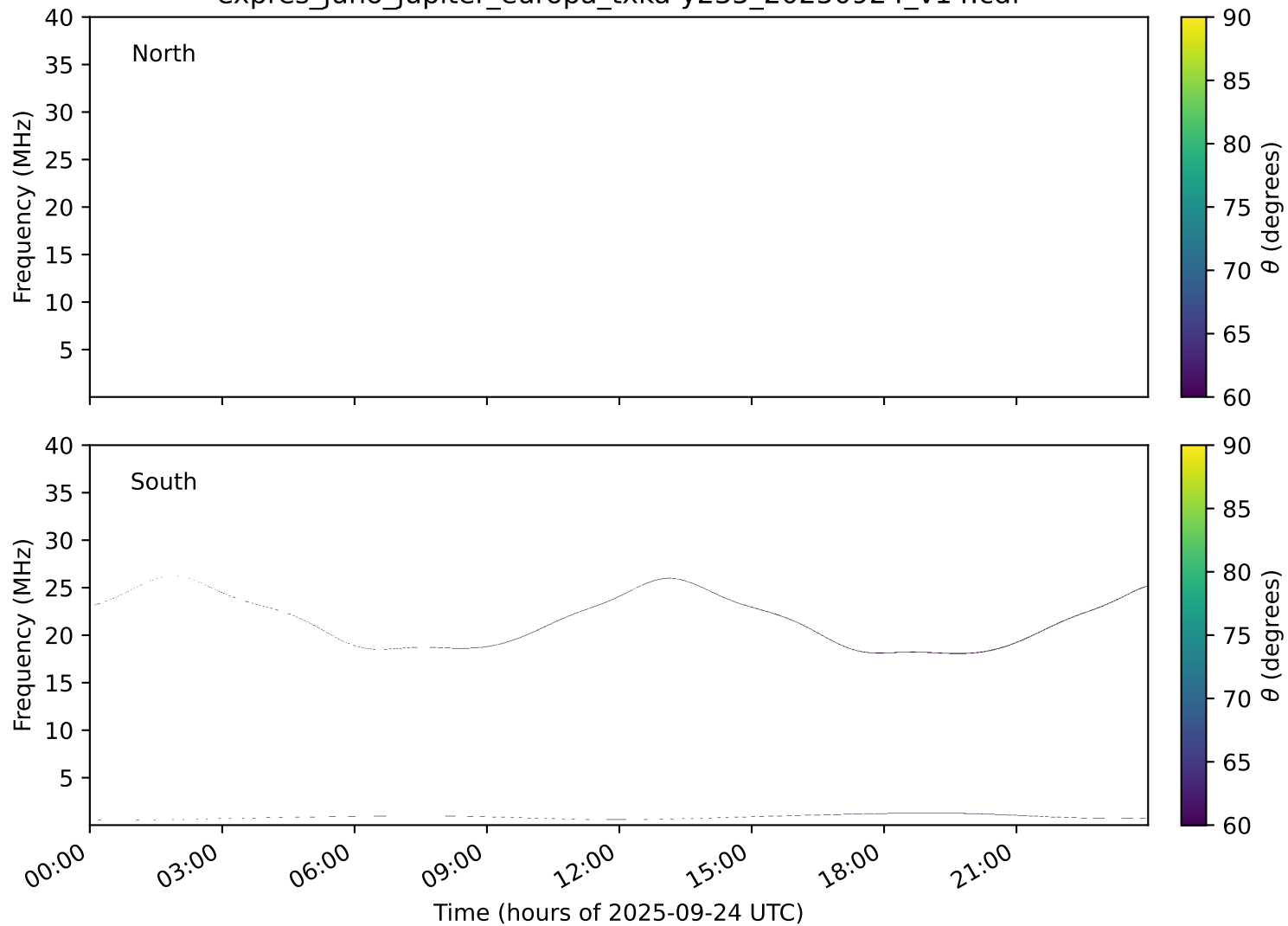
expres_juno_jupiter_europa_txka-y235_20250924_v14.cdf
