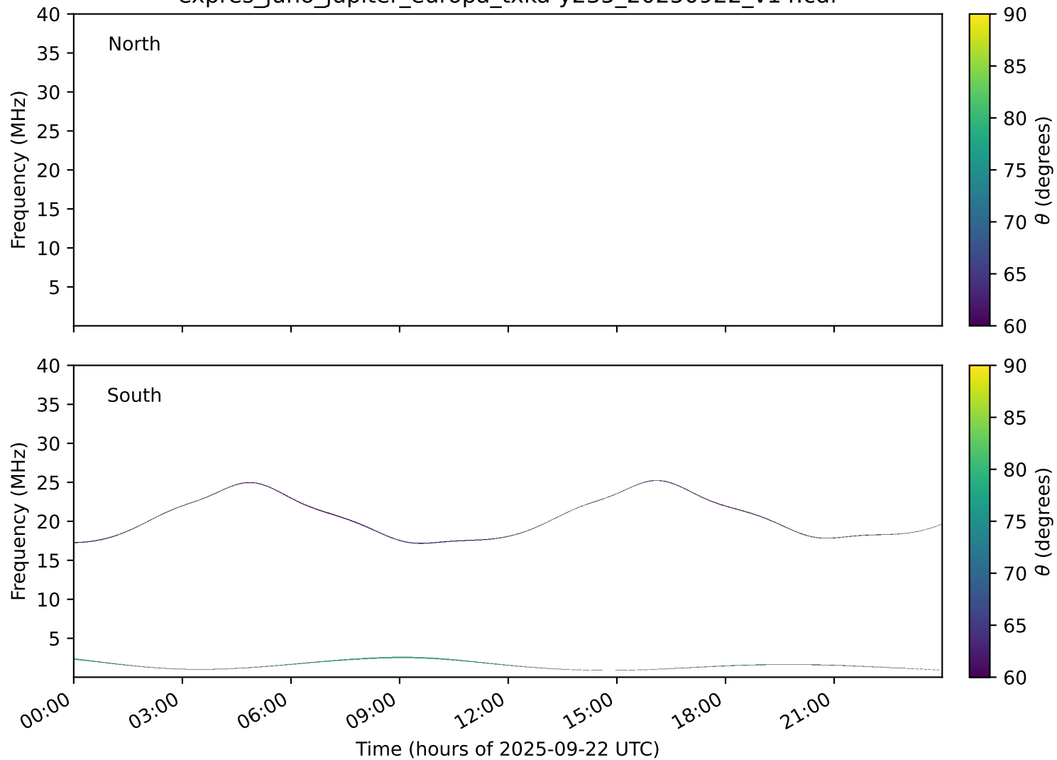
expres_juno_jupiter_europa_txka-y235_20250922_v14.cdf
