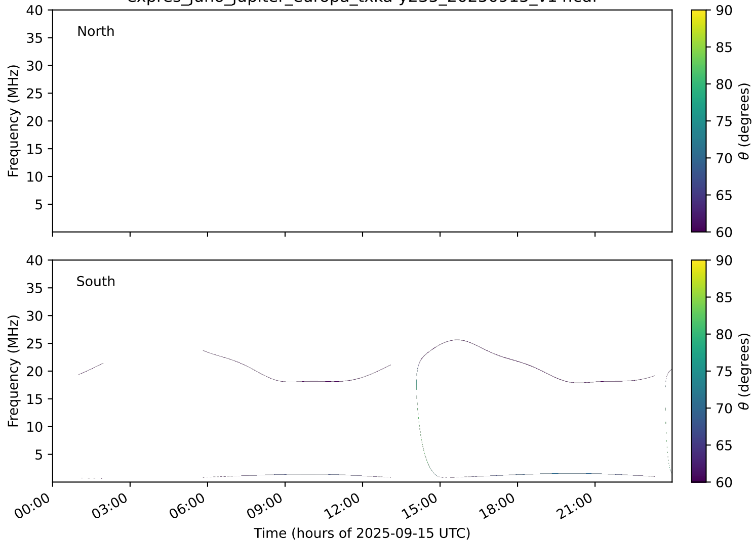
expres_juno_jupiter_europa_txka-y235_20250915_v14.cdf
