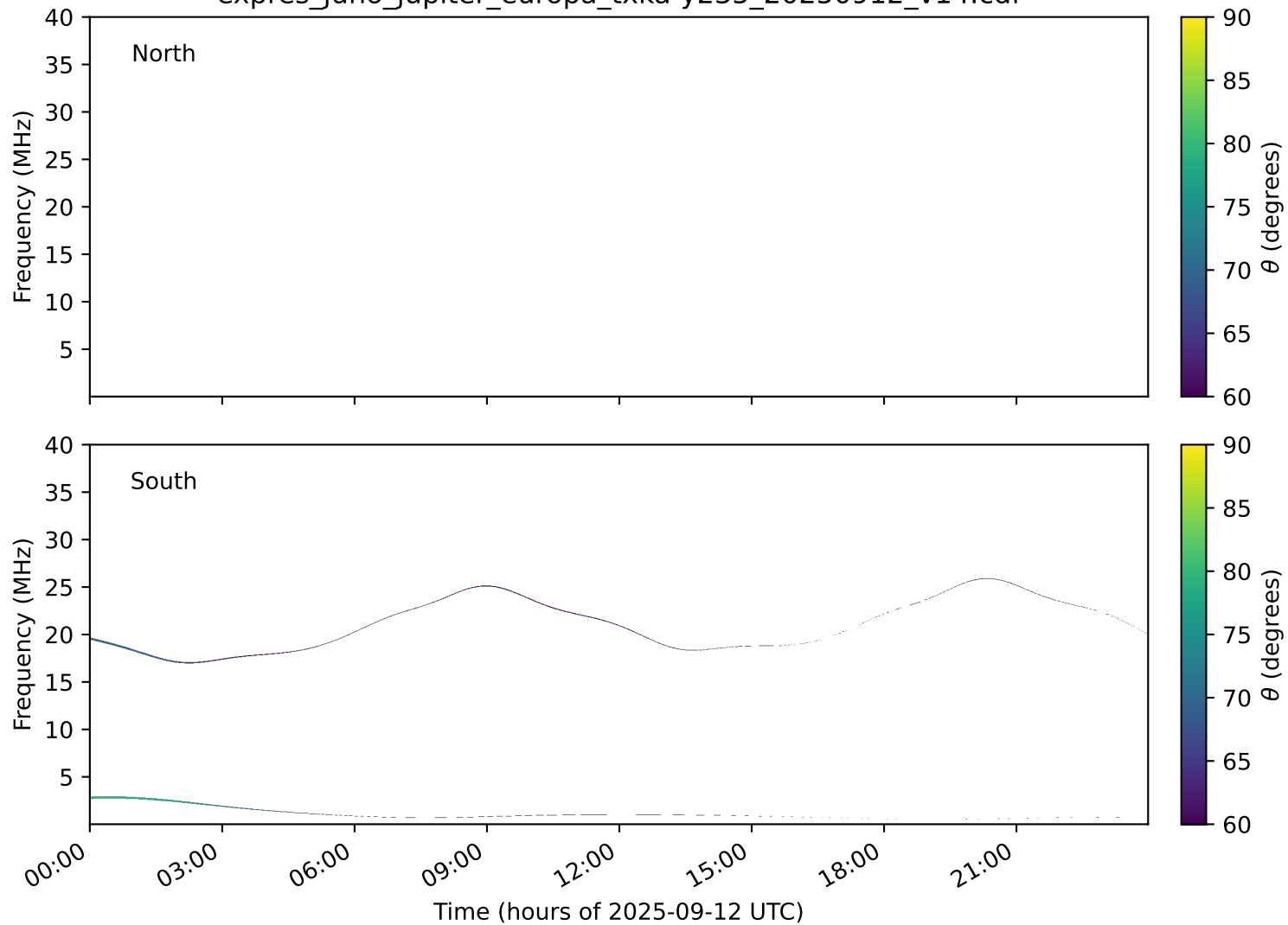
expres_juno_jupiter_europa_txka-y235_20250912_v14.cdf
