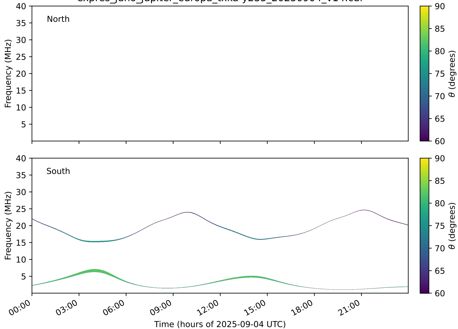
expres_juno_jupiter_europa_txka-y235_20250904_v14.cdf
