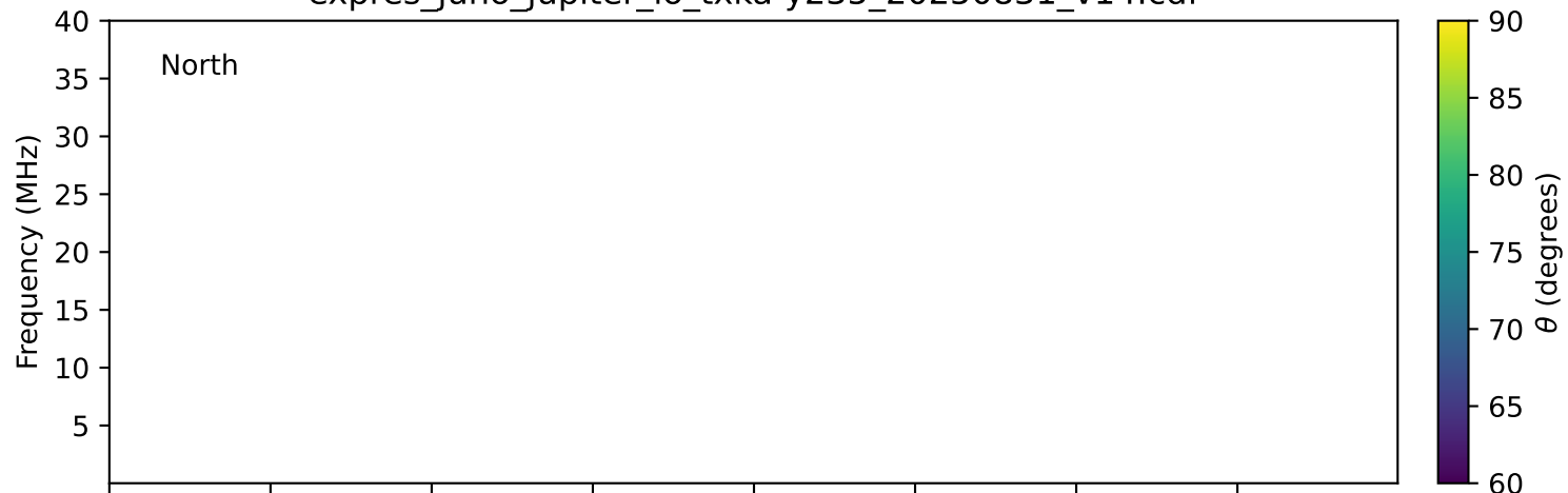
expres_juno_jupiter_io_txka-y235_20250831_v14.cdf
