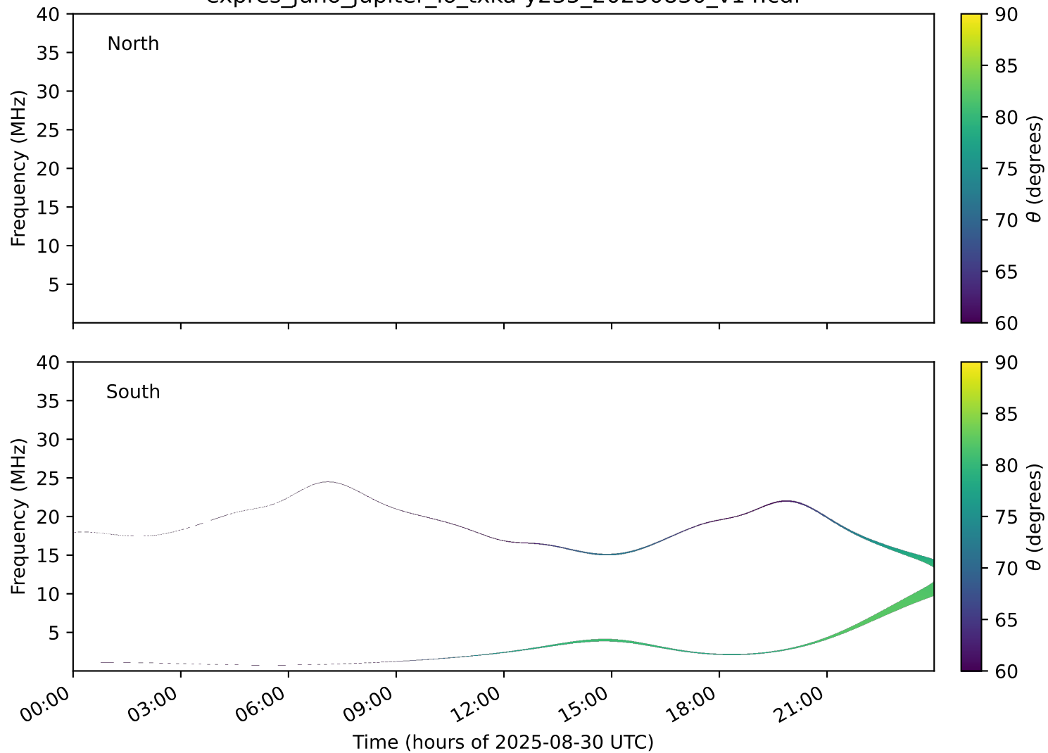
expres_juno_jupiter_io_txka-y235_20250830_v14.cdf
