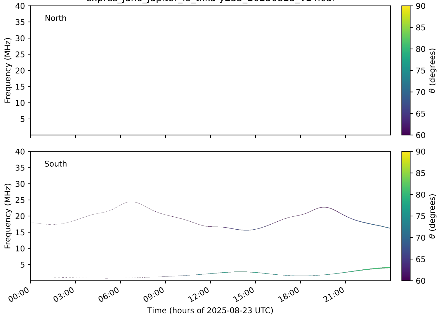
expres_juno_jupiter_io_txka-y235_20250823_v14.cdf
