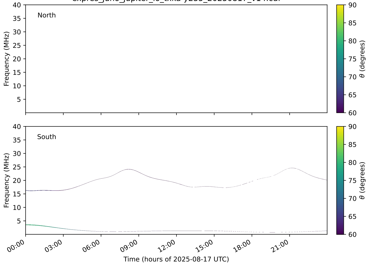
expres_juno_jupiter_io_txka-y235_20250817_v14.cdf
