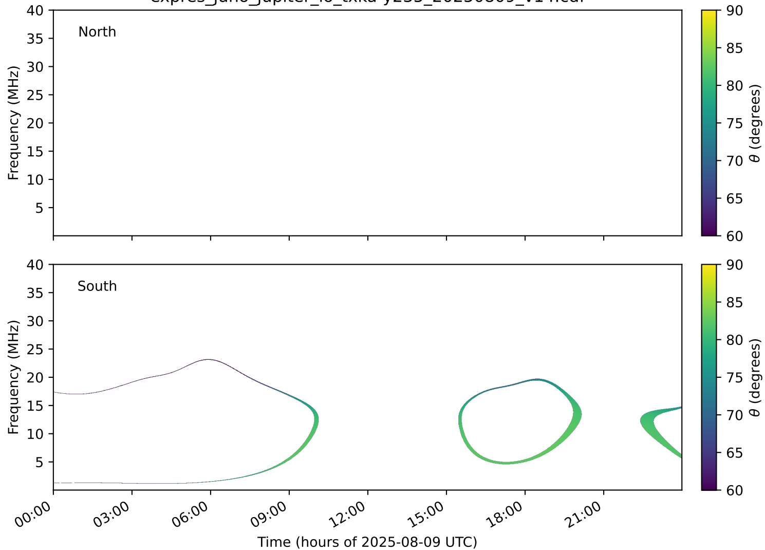
expres_juno_jupiter_io_txka-y235_20250809_v14.cdf
