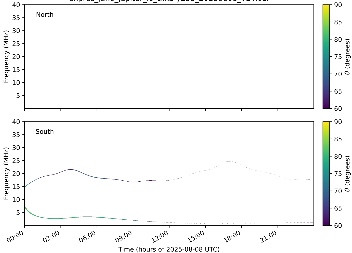
expres_juno_jupiter_io_txka-y235_20250808_v14.cdf
