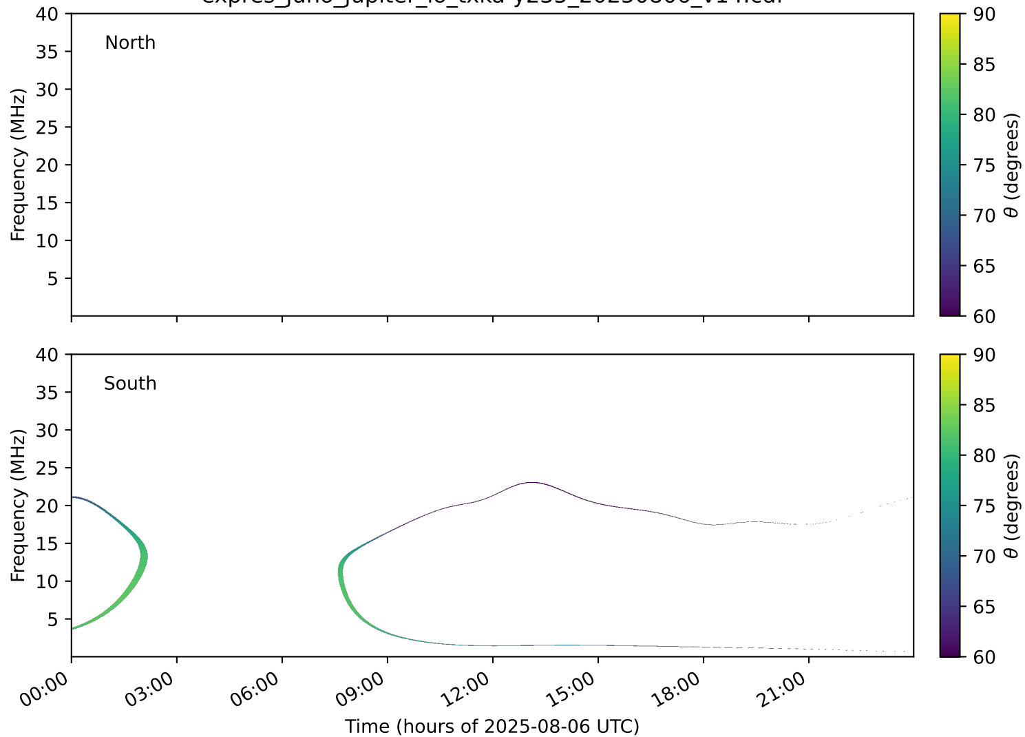
expres_juno_jupiter_io_txka-y235_20250806_v14.cdf
