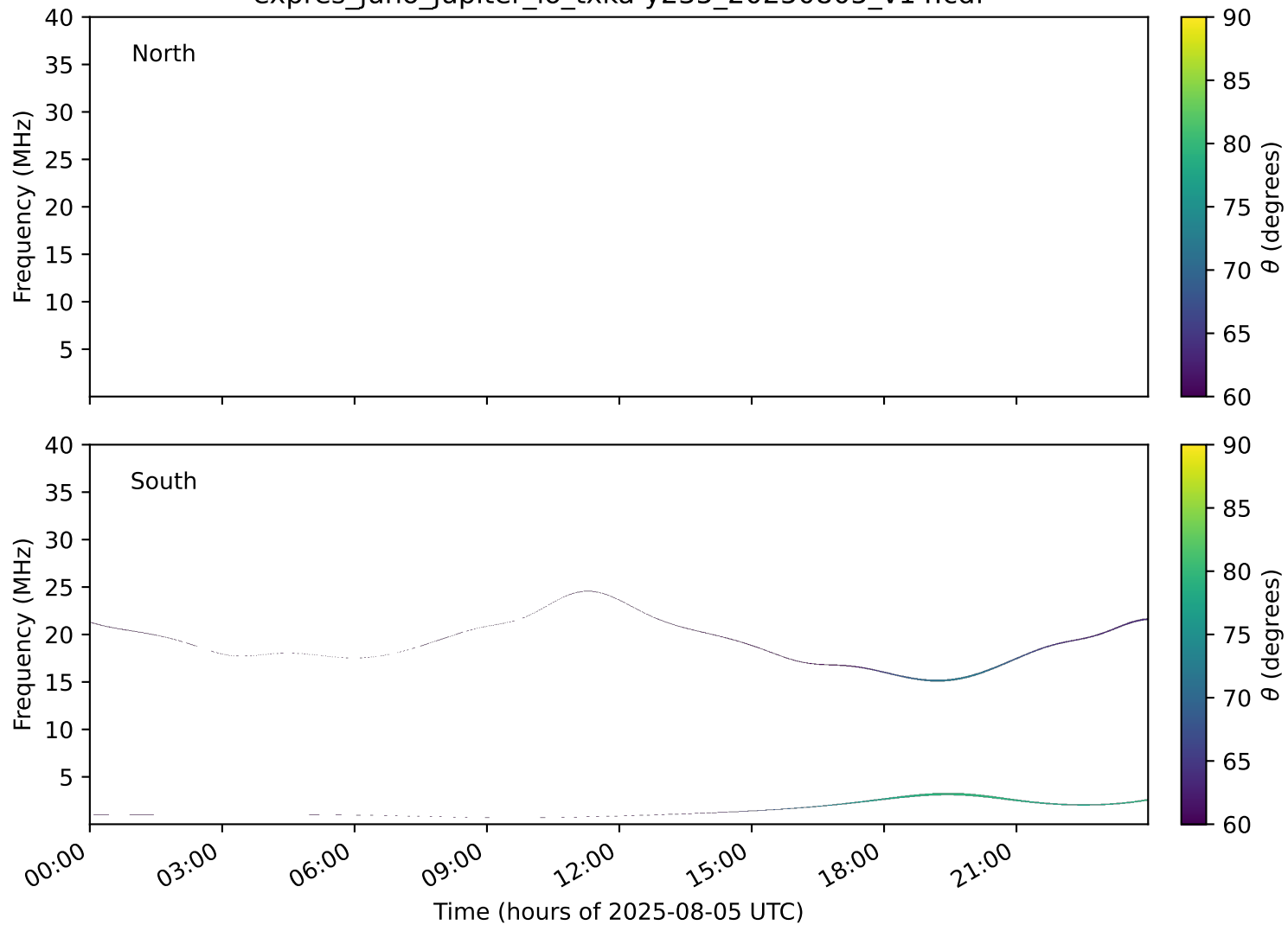
expres_juno_jupiter_io_txka-y235_20250805_v14.cdf
