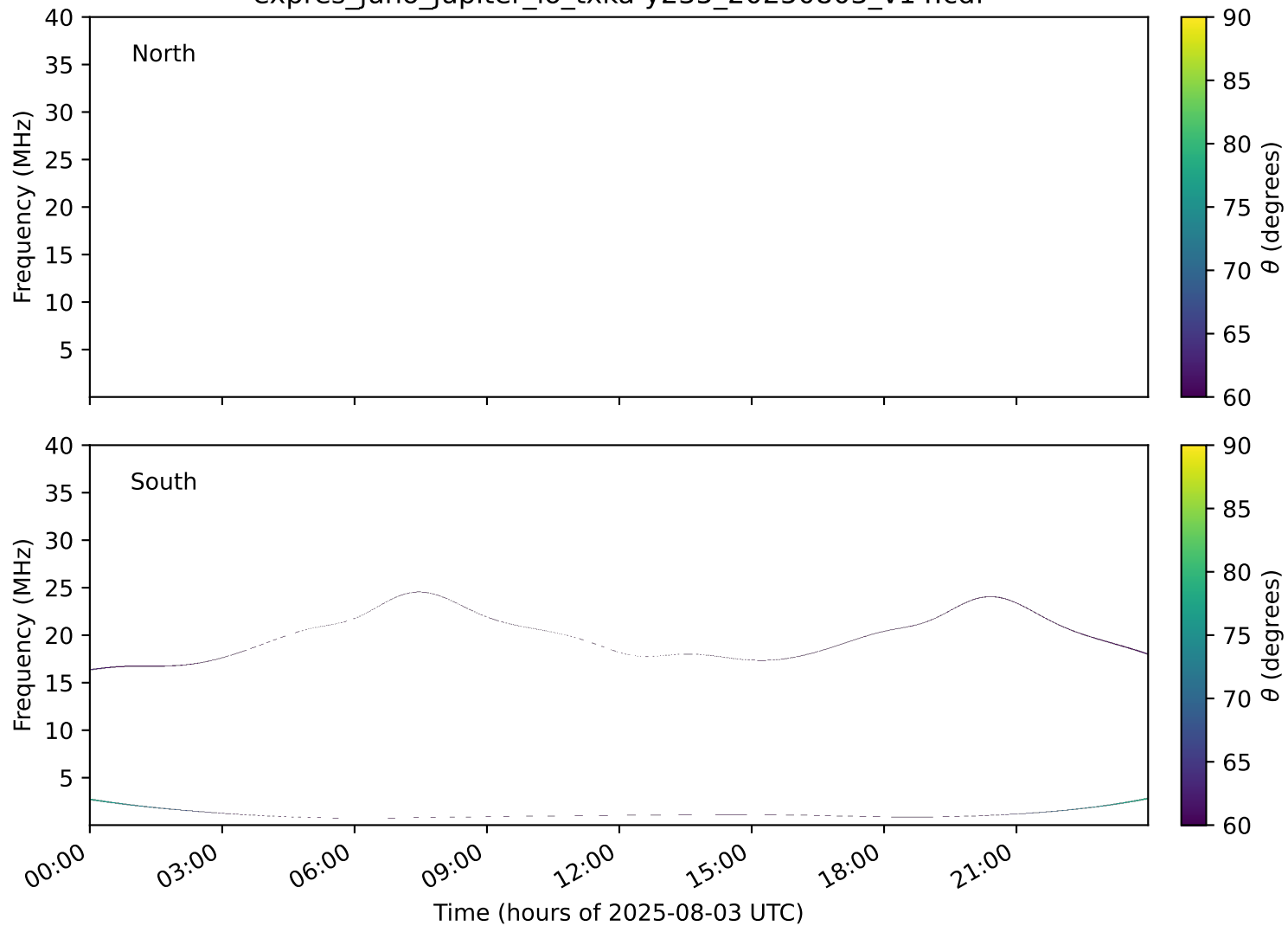
expres_juno_jupiter_io_txka-y235_20250803_v14.cdf
