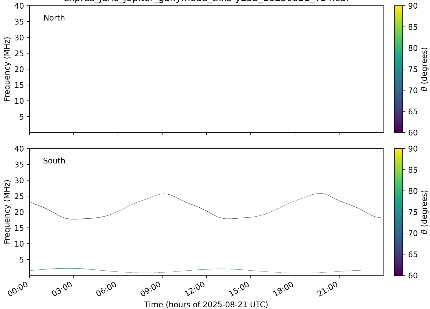
expres_juno_jupiter_ganymede_txka-y235_20250821_v14.cdf
