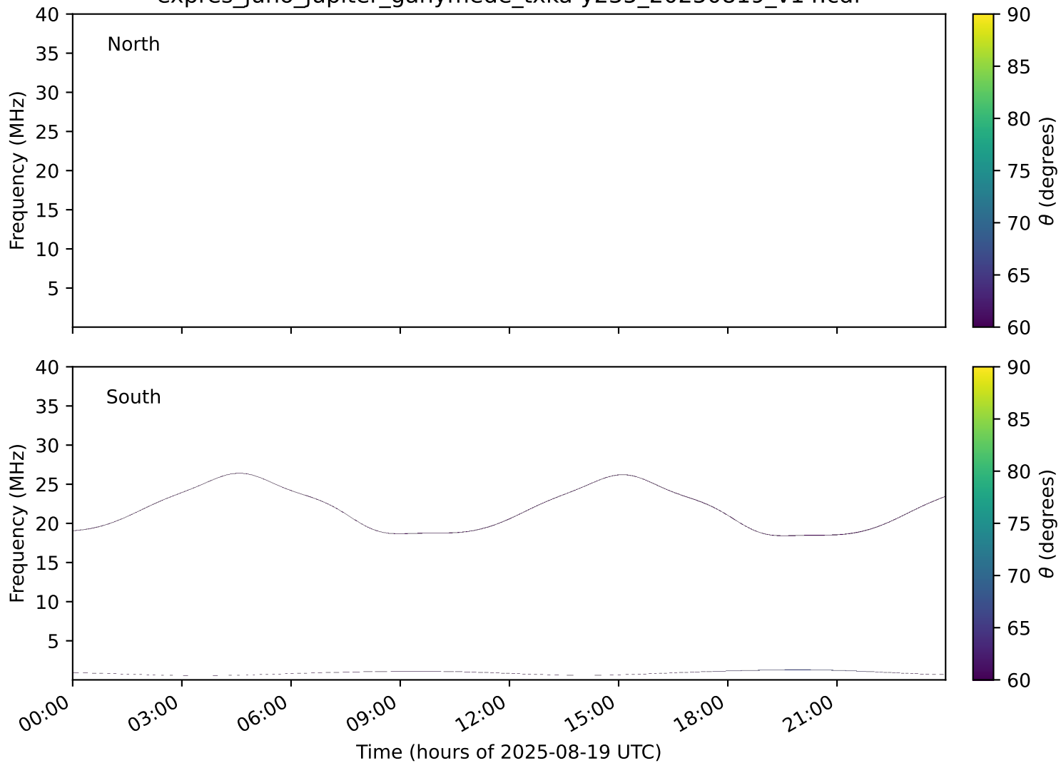
expres_juno_jupiter_ganymede_txka-y235_20250819_v14.cdf
