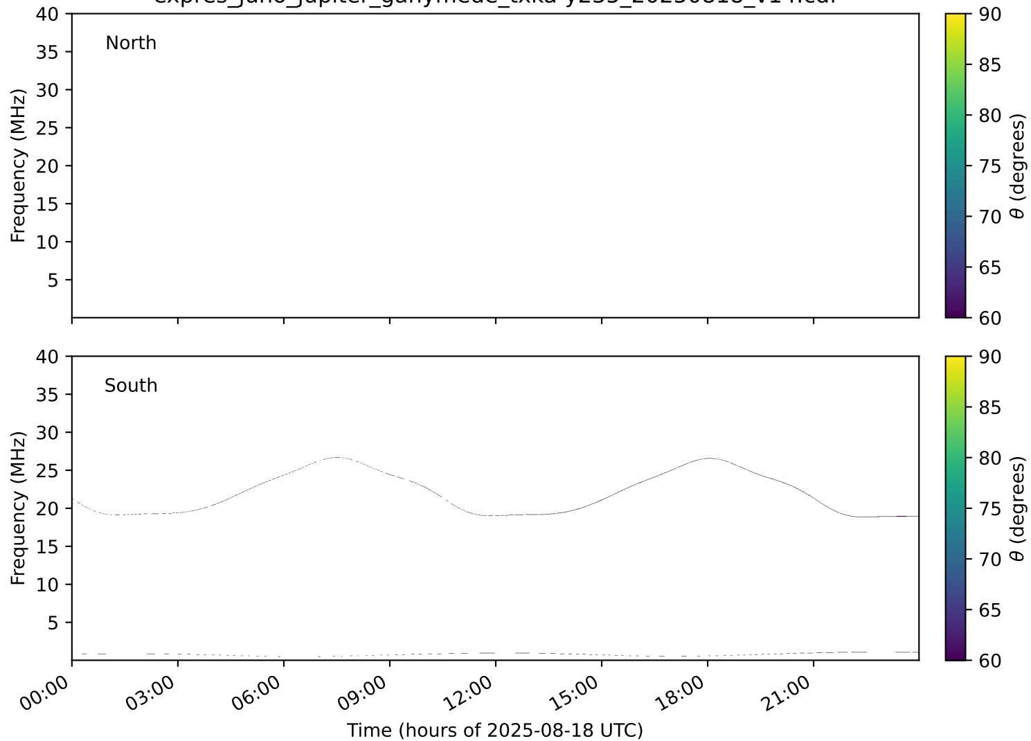
expres_juno_jupiter_ganymede_txka-y235_20250818_v14.cdf
