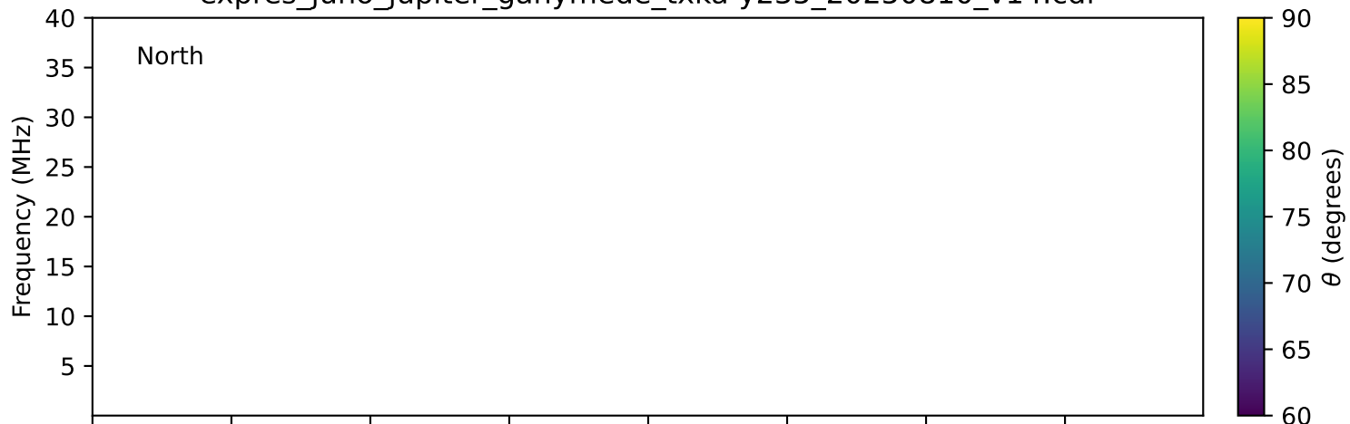
expres_juno_jupiter_ganymede_txka-y235_20250810_v14.cdf
