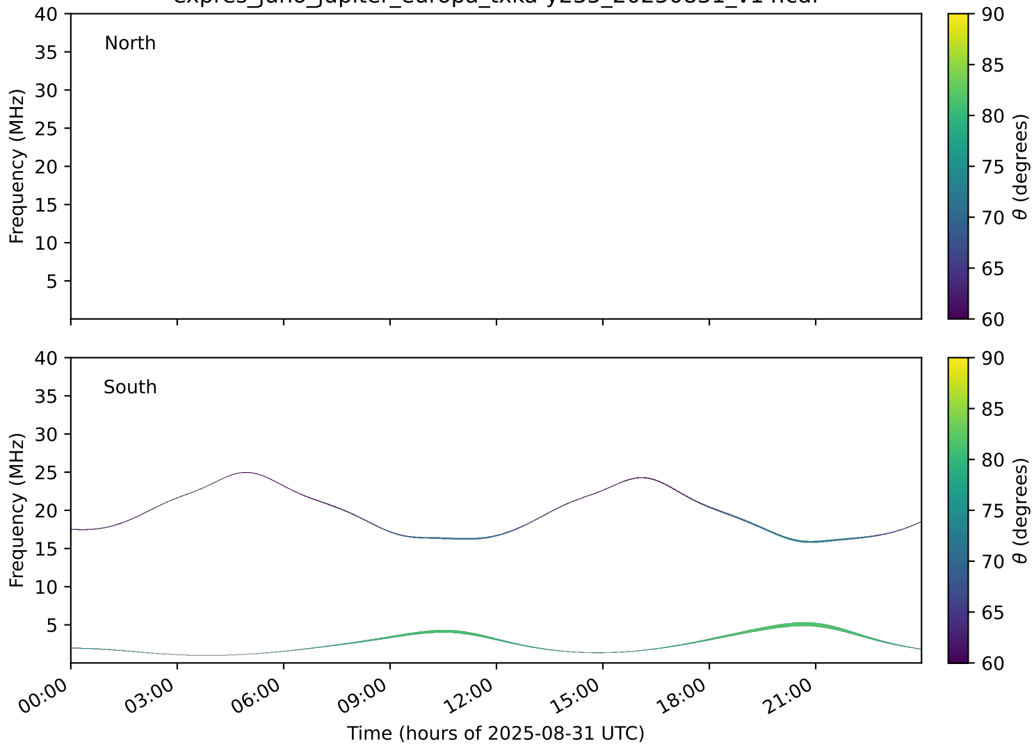
expres_juno_jupiter_europa_txka-y235_20250831_v14.cdf
