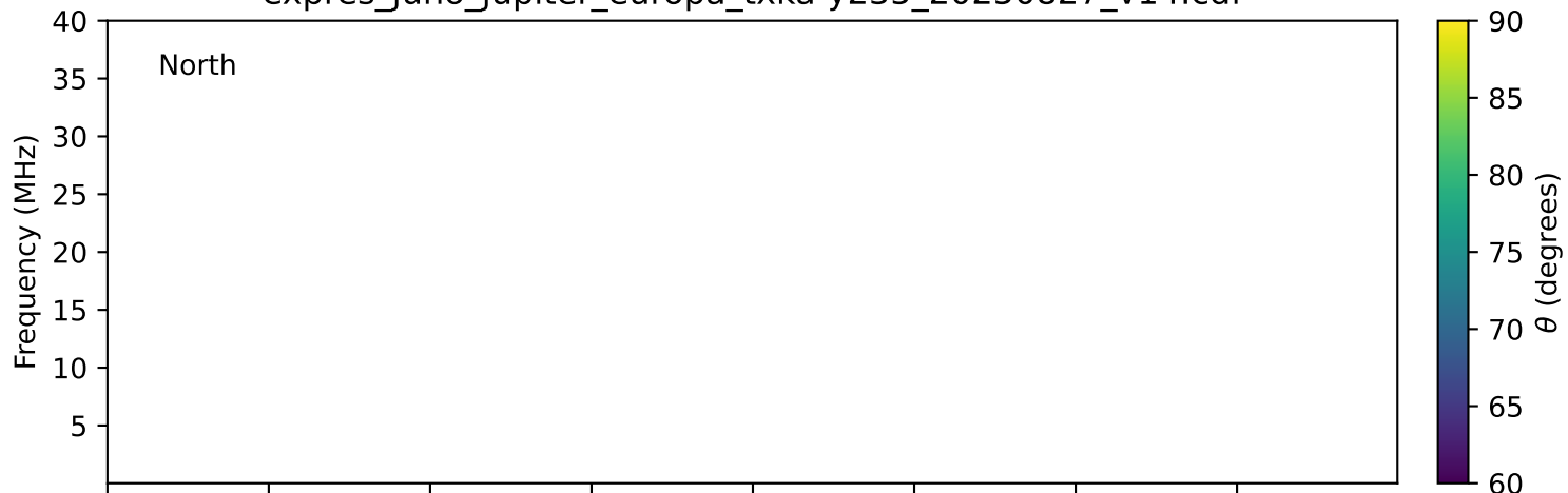
expres_juno_jupiter_europa_txka-y235_20250827_v14.cdf
