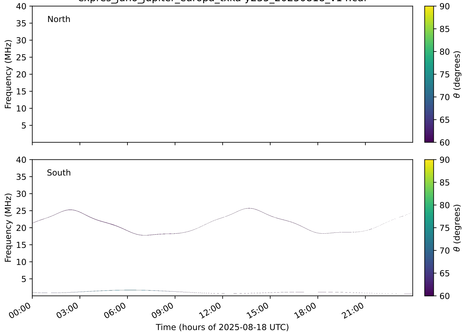
expres_juno_jupiter_europa_txka-y235_20250818_v14.cdf
