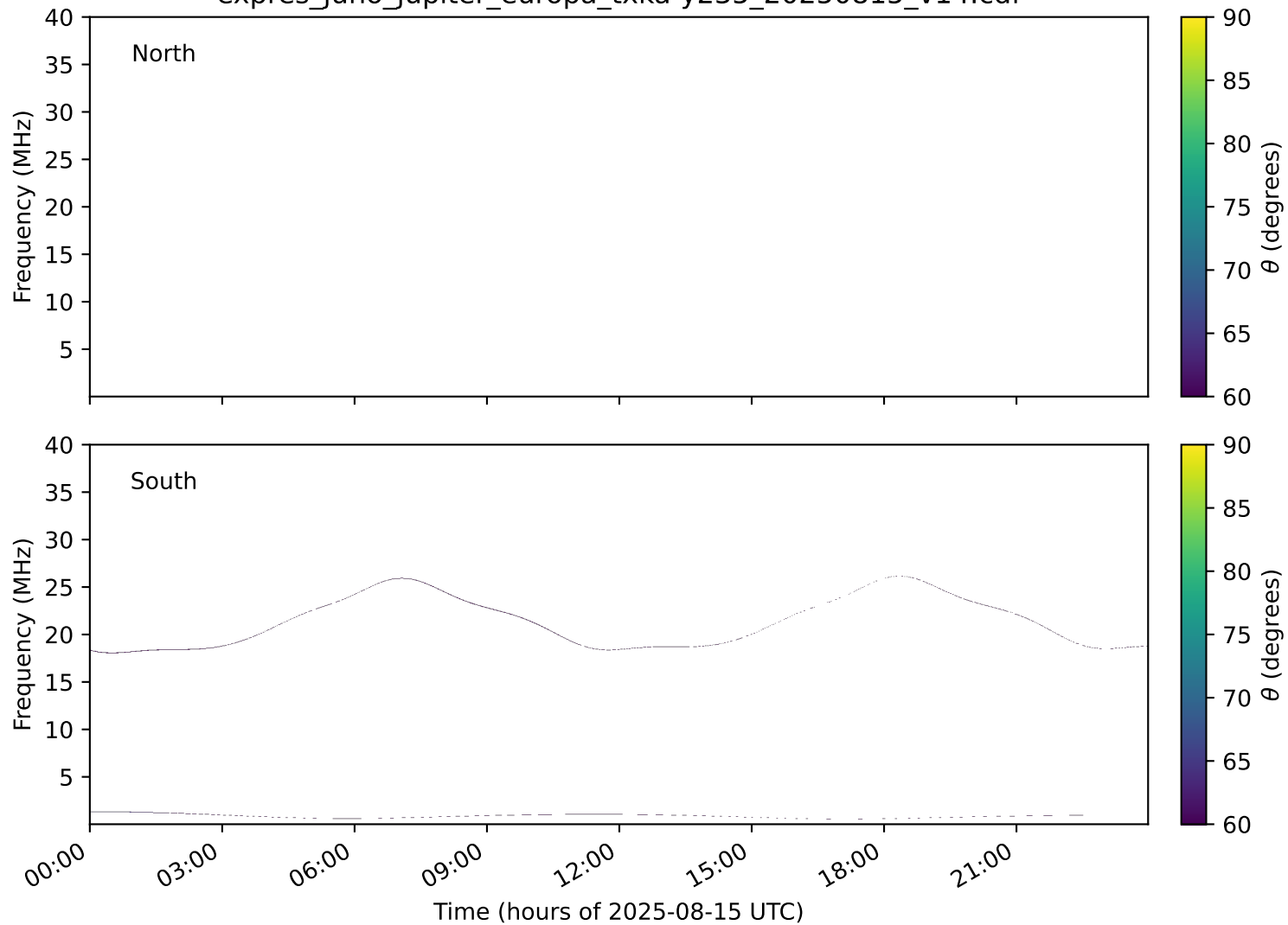
expres_juno_jupiter_europa_txka-y235_20250815_v14.cdf
