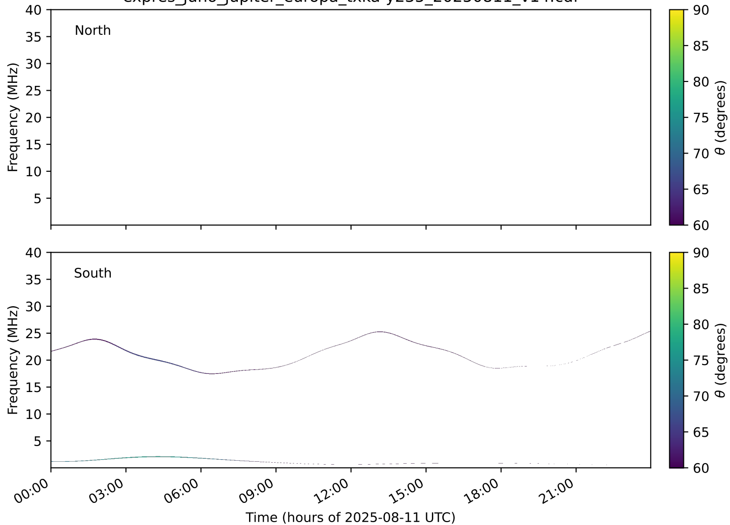
expres_juno_jupiter_europa_txka-y235_20250811_v14.cdf
