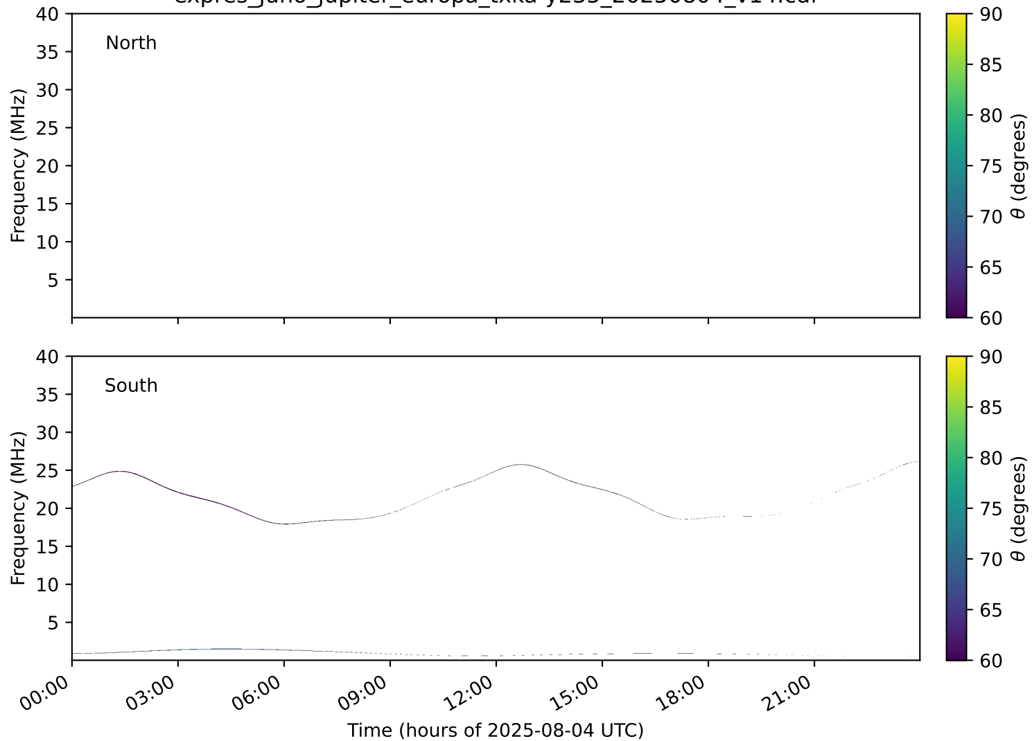
expres_juno_jupiter_europa_txka-y235_20250804_v14.cdf
