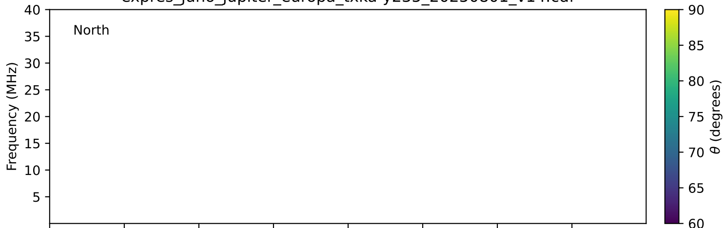
expres_juno_jupiter_europa_txka-y235_20250801_v14.cdf
