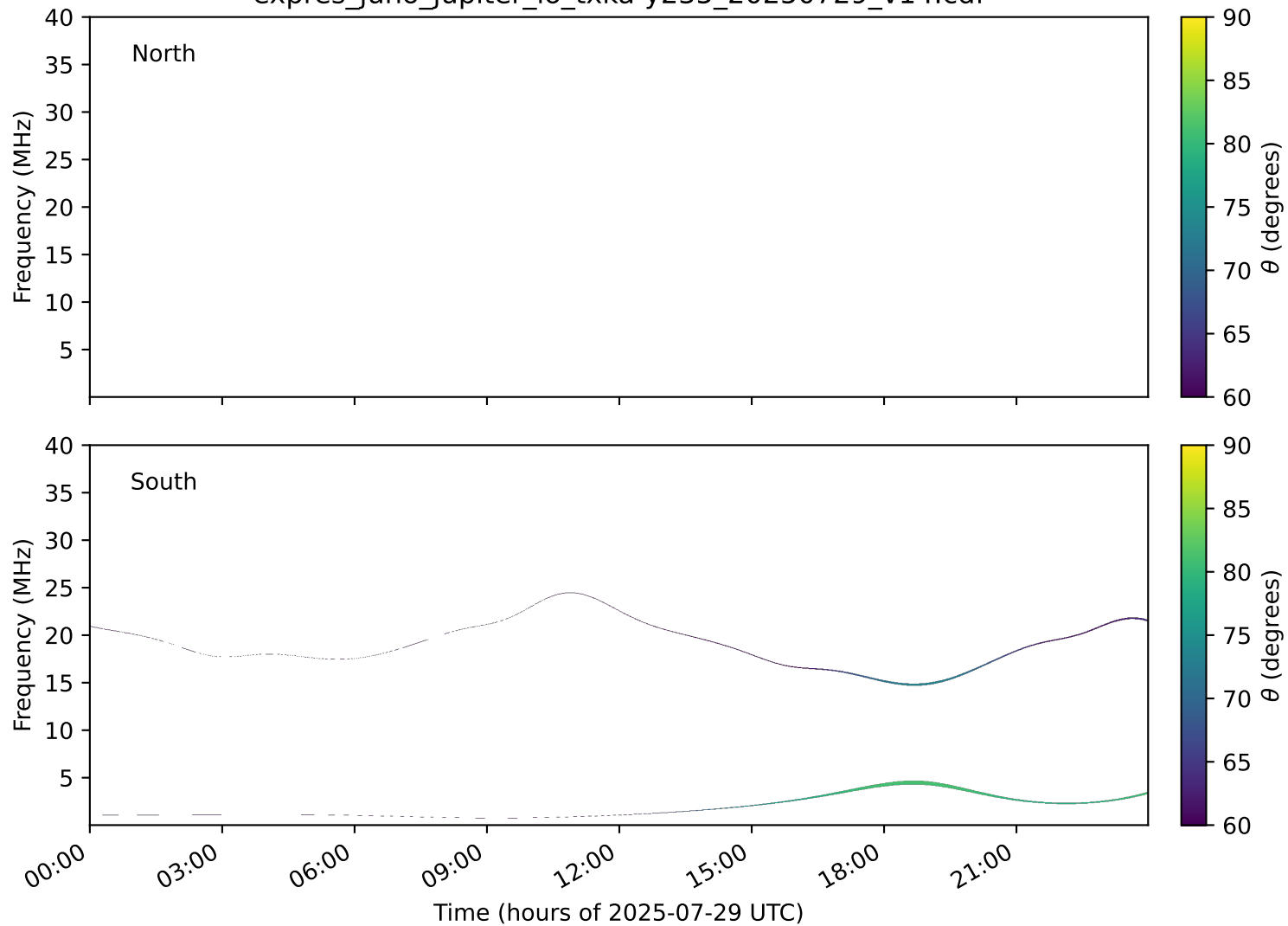
expres_juno_jupiter_io_txka-y235_20250729_v14.cdf
