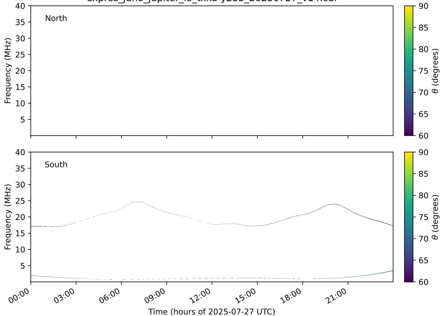
expres_juno_jupiter_io_txka-y235_20250727_v14.cdf
