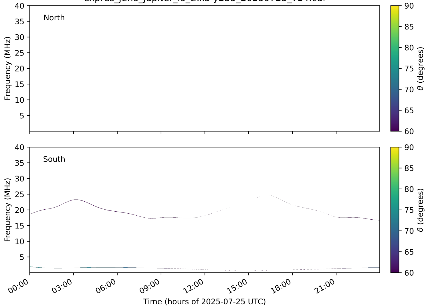
expres_juno_jupiter_io_txka-y235_20250725_v14.cdf
